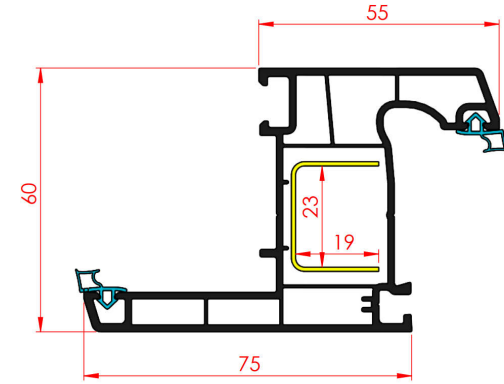
60 mm 3 odacıklı Pervazlı Kasa Profili 60 mm 3 Chambered Frame Profile
