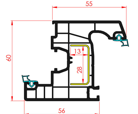
60 mm 4 odacıklı Kanat Profili 60 mm 4 Chamber Wing Profile
