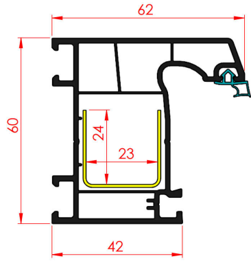
60 mm 3 odacıklı L Kasa Profili 60 mm 3 Chamber L Frame Profile
