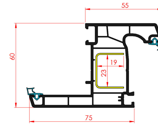
60 mm 4 odacıklı Pervazlı Kasa Profili 60 mm 4 Chambered Frame Profile
