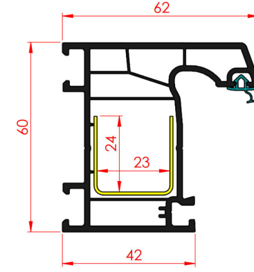
60 mm 4 odacıklı L Kasa Profili 60 mm 4 Chamber L Frame Profile
