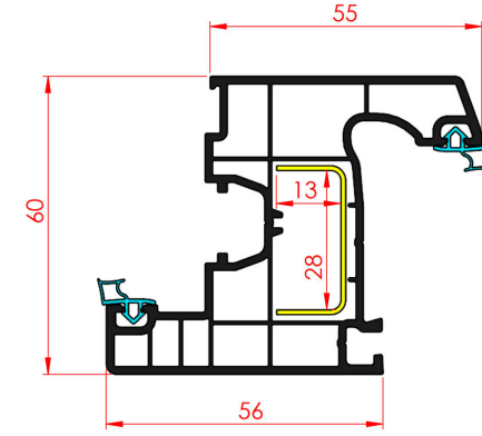
60 mm 3 odacıklı Kanat Profili 60 mm 3 Chamber Wing Profile
